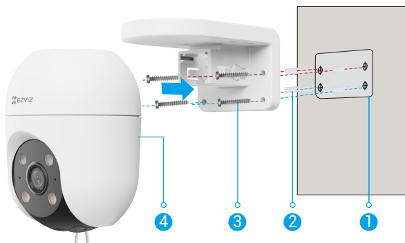
Fig. 2 Wall Mount
